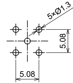
RECOMMENDED PCB MOUNTING HOLE
