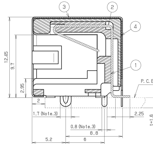
嵌合部詳細 (S=5/1) Contact detail (S=5/1)
