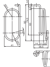
NPCH-4183R
