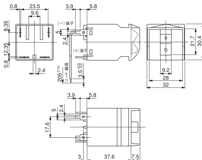
<HAS-P-40>
