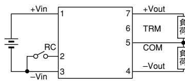
CC6-xxxxDx-E
