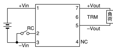
CC6-xxxxSx-E
